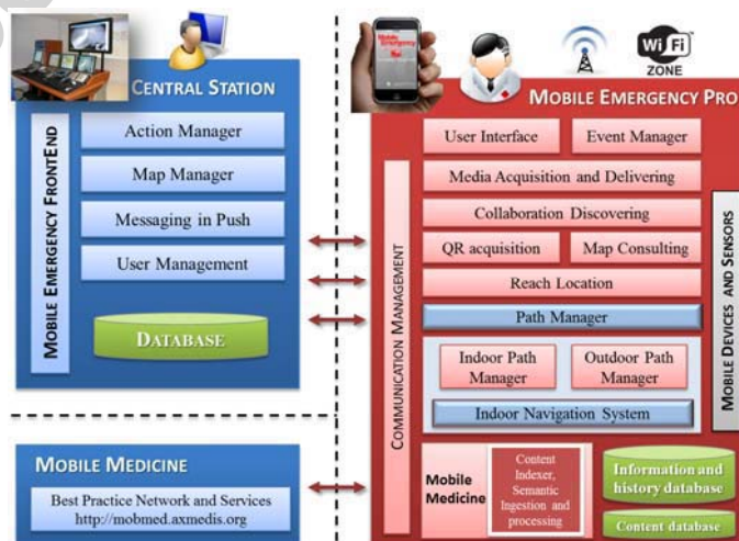
Figure 1. Architecture of the Mobile Emergency Pro solution
