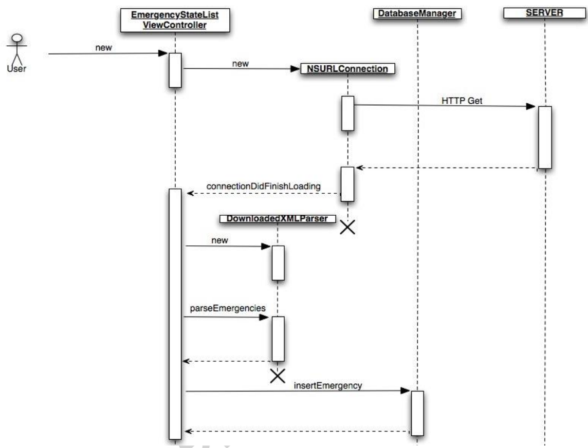
Figure 2 - UML Diagram sequence: recovery of emergencies status
