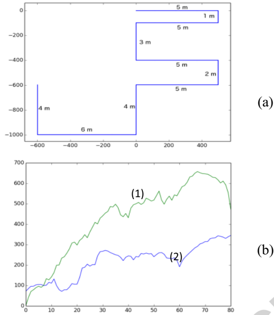
Figure 6 - (a) the indoor path for test (starting from the entrance and exploring some of the rooms, thus multiple changes of directions), (b) trend of the mean error of estimated for navigation with (1) dead reckoning, (2) Kalman filtering. Error is in mm and the path length was of 40 mt.
