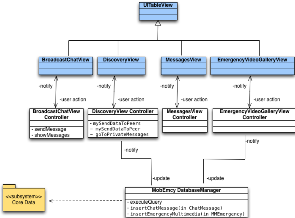
Figure 3 - UML Diagram regarding collaboration discovering aspects
