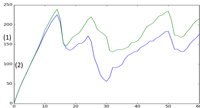
Figure 8 - Trend of the mean error of estimated positions during navigation for (1) Extended Kalman, (2) Adaptive Extended Kalman filtering. Errors is in mm.
