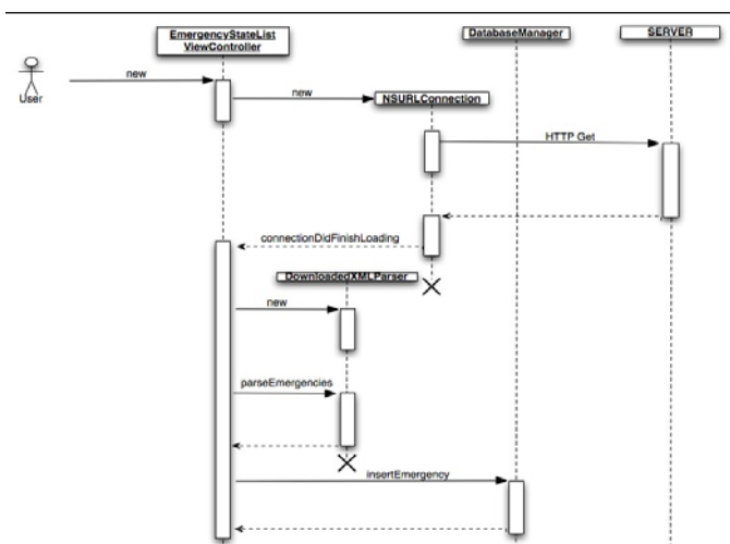
Figure 2 - UML Diagram sequence: recovery of emergencies status
