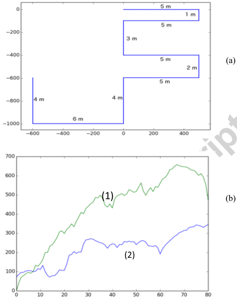
Figure 6 - (a) the indoor path for test (starting from the entrance and exploring some of the rooms, thus multiple changes of directions), (b) trend of the mean error of estimated for navigation with (1) dead reckoning, (2) Kalman filtering. Error is in mm and the path length was of 40 mt.
