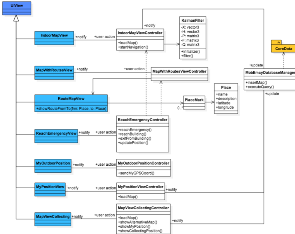
Figure 5 - UML Diagram regarding integrated navigation aspects.
